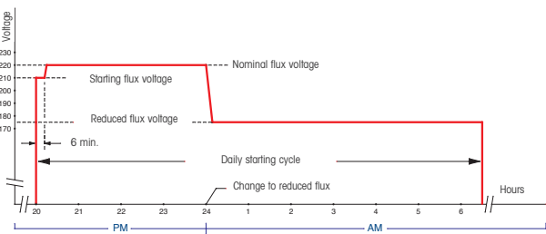
Equipment start-up regime curve, rating, and reduced until sunrise of the ESDONI equipment..
