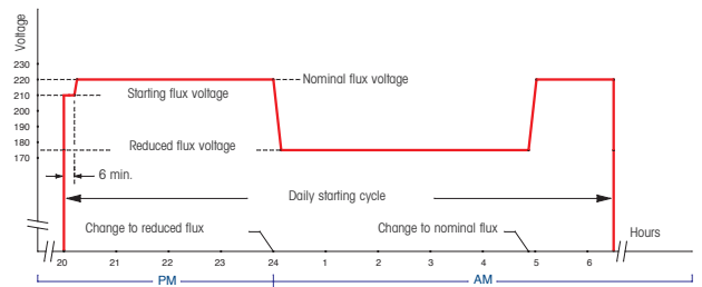
Start-up regime curve, rating, reduced and return to the rating regime of the ESDONI equipment.
