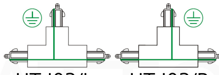
HT-J03/L HT-J03/R
